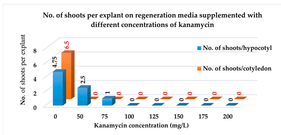
Figure 10. Number of shoots per explant on regeneration media supplemented with different concentrations of kanamycin.
