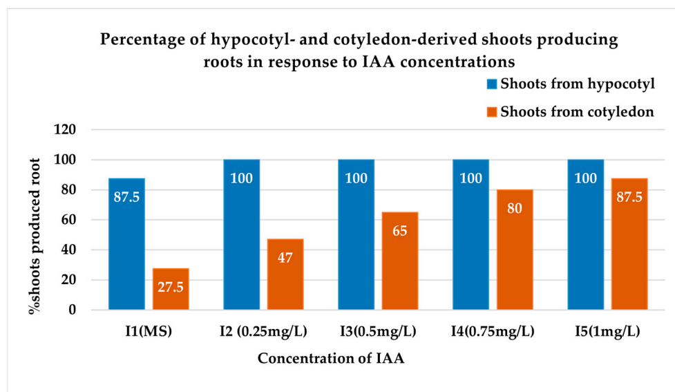
Figure 5. Percentage of hypocotyl- and cotyledon-derived shoots producing roots on MS media supplemented with different IAA concentrations.
