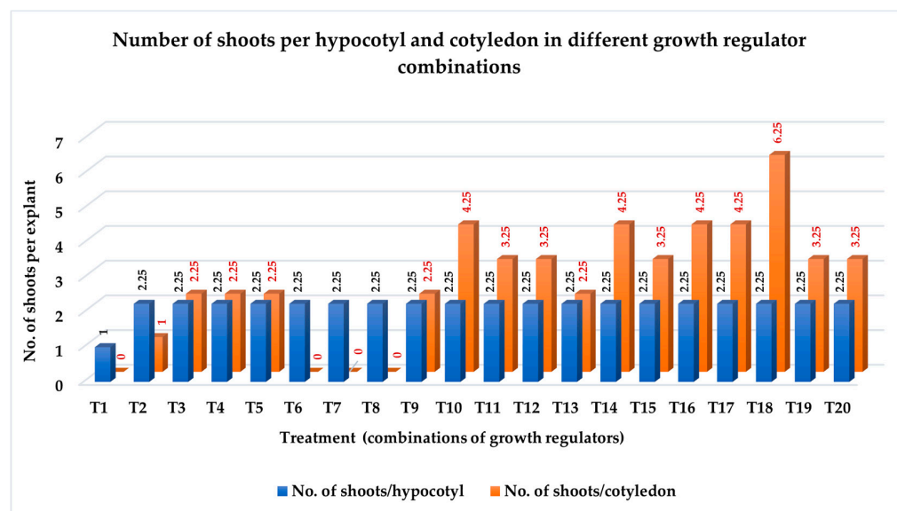
Figure 2. Number of shoots per hypocotyl and cotyledon explants on MSB5 supplemented with different concentration combinations of BAP and IAA.
