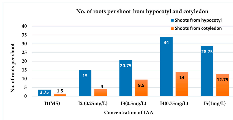
Figure 6. Number of roots per shoot derived from hypocotyl and cotyledon explants on MS media supplemented with different IAA concentrations.
