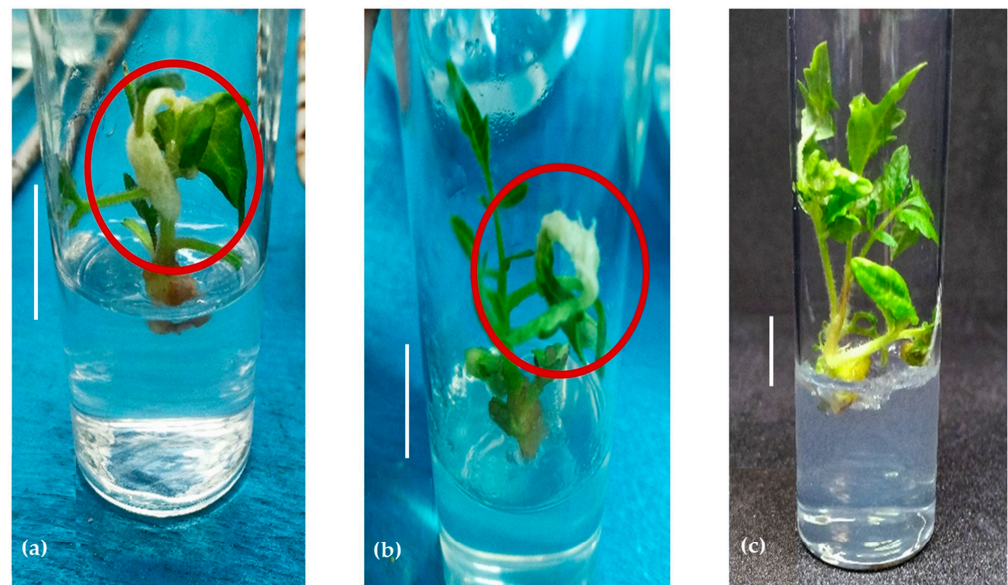
Figure 4. Elongation of regenerated shoots. (a) Callus (near the shoot tip) growing on the shoot in MS +2 mg/L BAP +0.1 mg/L IAA; (b) callus (on leaves) growing on shoot MS +2 mg/L BAP +0.1 mg/L IAA; (c) normal growth of shoots on MS medium without PGR. Scale bar = 2 cm.
