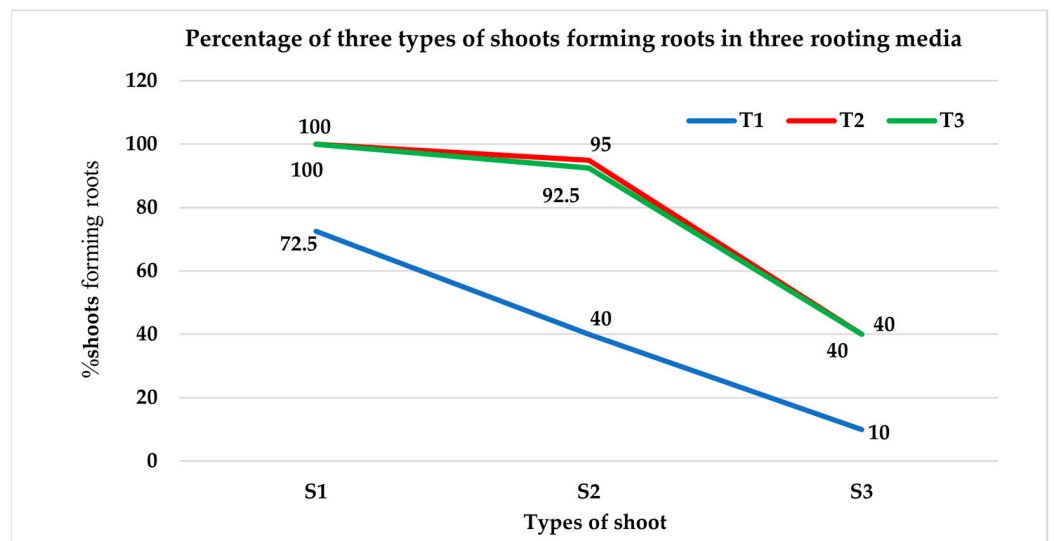
Figure 11. Percentage of three types of shoots forming roots on three rooting media.
