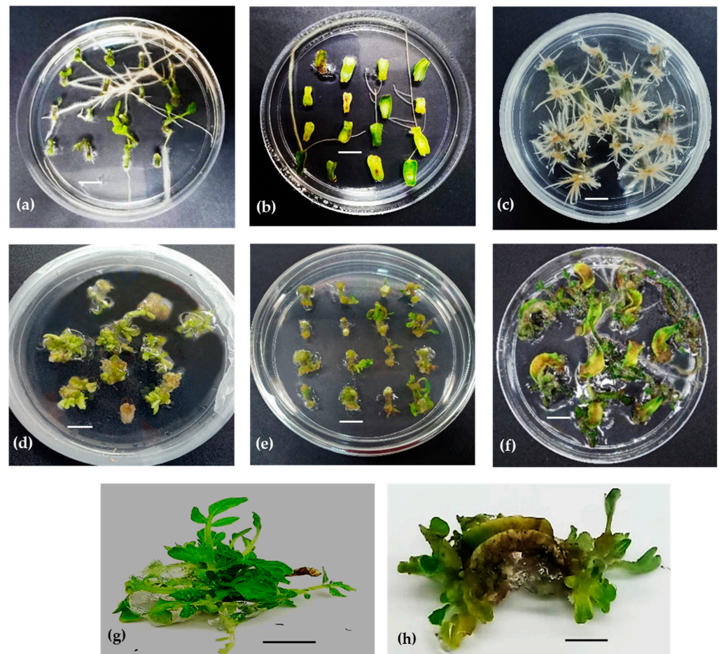
Figure 3. Regeneration of shoots from cotyledon and hypocotyl explants of tomato cv. MT1 under different concentration combinations of BAP and IAA: (a) HT1 induced roots and shoots (scale bar: 1 cm); (b) CT1 induced only roots (scale bar: 1 cm); (c) CT8 induced only roots (scale bar: 1 cm); (d) E1T4 induced more leaves than calli than shoot (scale bar: 1 cm); (e) HT14 induced multiple shoots, roots, and leaves (scale bar: 1 cm); (f) CT18 induced multiple shoots, roots, and leaves (scale bar: 1 cm); (g) multiple shoots regenerated from hypocotyls (scale bar, 0.5 cm); (h) multiple shoots regenerated from cotyledons (scale bar, 0.5 cm). H = hypocotyls, C = cotyledons, T1 = MSB5 + 0 mg/L BAP + 0 mg/L IAA, T4 = MSB5 + 3 mg/L BAP + 0.0 mg/L IAA, T8 = MSB5 + 0 mg/L BAP + 0.5 mg/L IAA, T14 = MSB5 + 2 mg/L BAP + 0.1 mg/L IAA, T18 = MSB5 + 2 mg/L BAP + 0.5 mg/L IAA.
