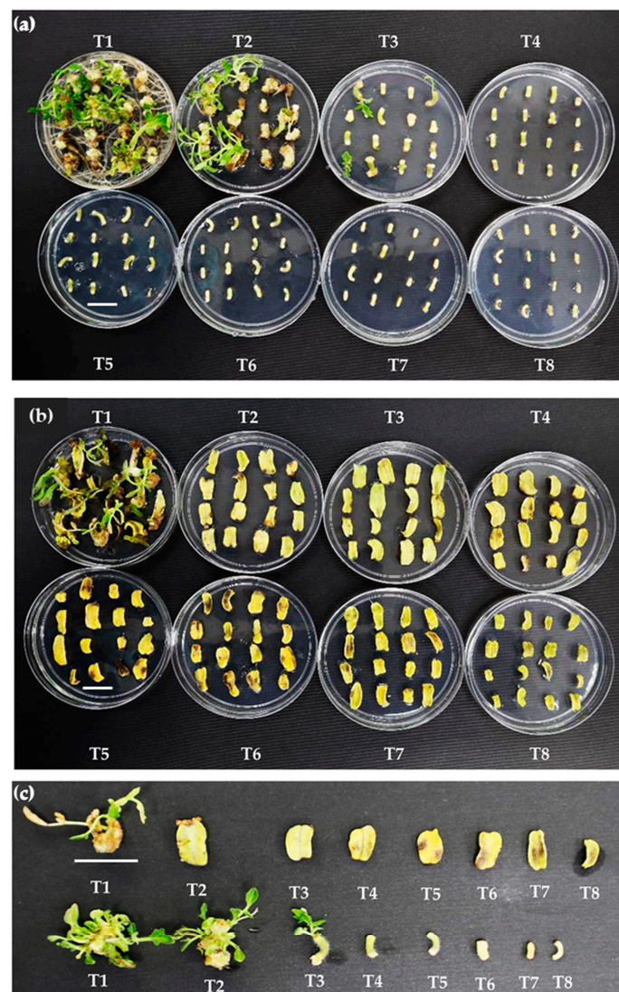
Figure 9. Response of tomato cv. MT1 explants to different kanamycin concentrations. (a) Response of hypocotyl explants; (b) response of cotyledon explants; (c) representative explants forming shoots. T1 = 0 mg/L, T2 = 50 mg/L, T3 = 75 mg/L, T4 = 100 mg/L, T5 = 125 mg/L, T6 = 150 mg/L, T7 = 175 mg/L, and T8 = 200 mg/L of kanamycin. Scale bar = 2 cm.
