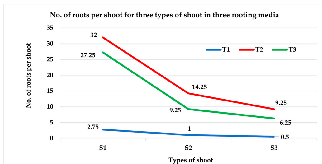
Figure 12. Number of roots per shoot for three types of shoots on three rooting media.
