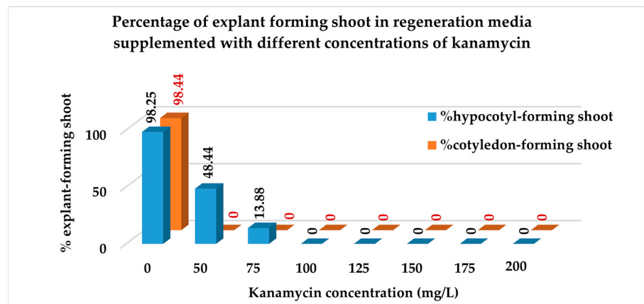
Figure 8. Percentage of explants forming shoots on regeneration media supplemented with different concentrations of kanamycin.
