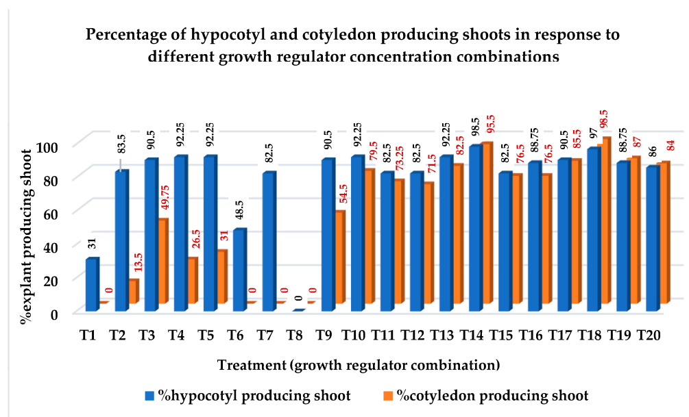
Figure 1. Percentage (%) of hypocotyl and cotyledon explants producing shoots on different concentration combinations of BAP and IAA in MSB5 medium.
