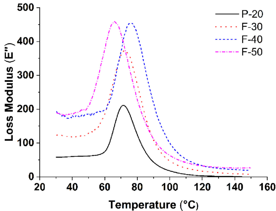
Fig. 3. Loss modulus of F-30, F-40, F-50 and P-20.
