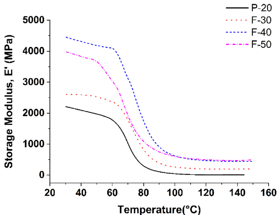
Fig. 2. Storage modulus of F-30, F-40, F-50 and P-20.
