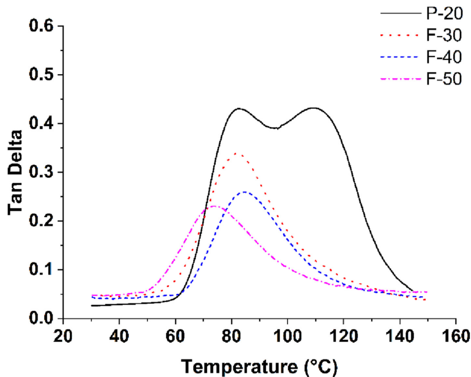
Fig. 4. Damping factor of F-30, F-40, F-50 and P-20.
