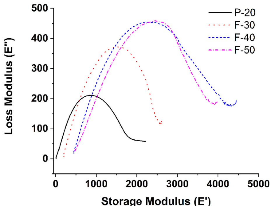
Fig. 5. Cole-cole plot of F-30, F-40, F-50 and P-20.
