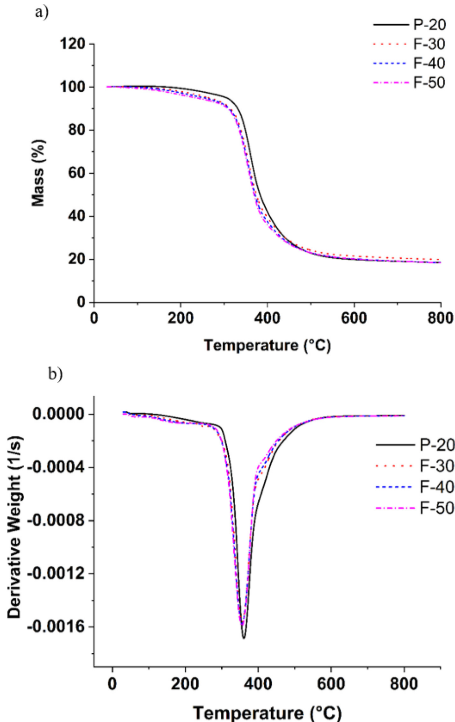
Fig. 6. TG and DTG plot of F-30, F-40, F-50 and P-20.
