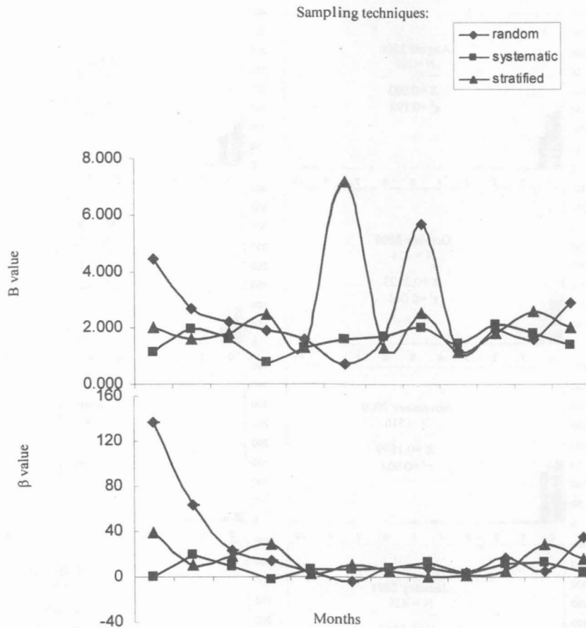
Fig. 4: Comparison of temporal variation of b and \beta values based on three different methods of sampling from August 2000 till September 2001
